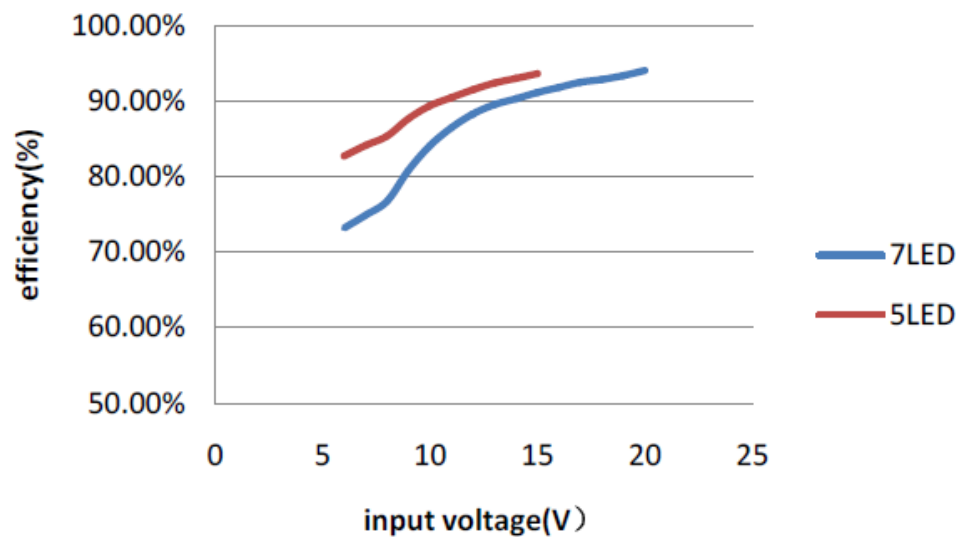
efficiency VS. input voltage
